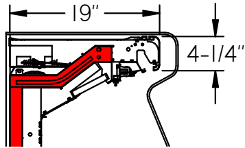
FLAT NOSE CANOPY
